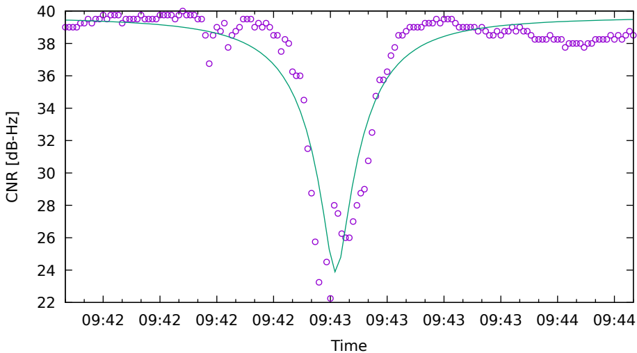
CNR fit for G08 on XiaomiMi8 - drive 14 (DOY262)
