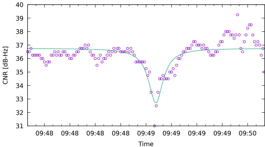
CNR fit for G08 on XiaomiMi8 - drive 17 (DOY262)
