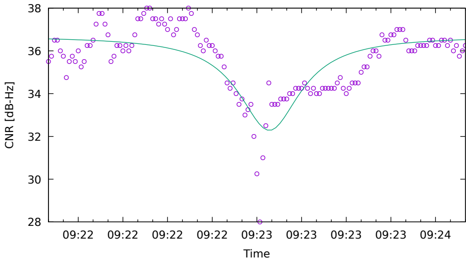
CNR fit for G08 on XiaomiMi8 - drive 4 (DOY262)
