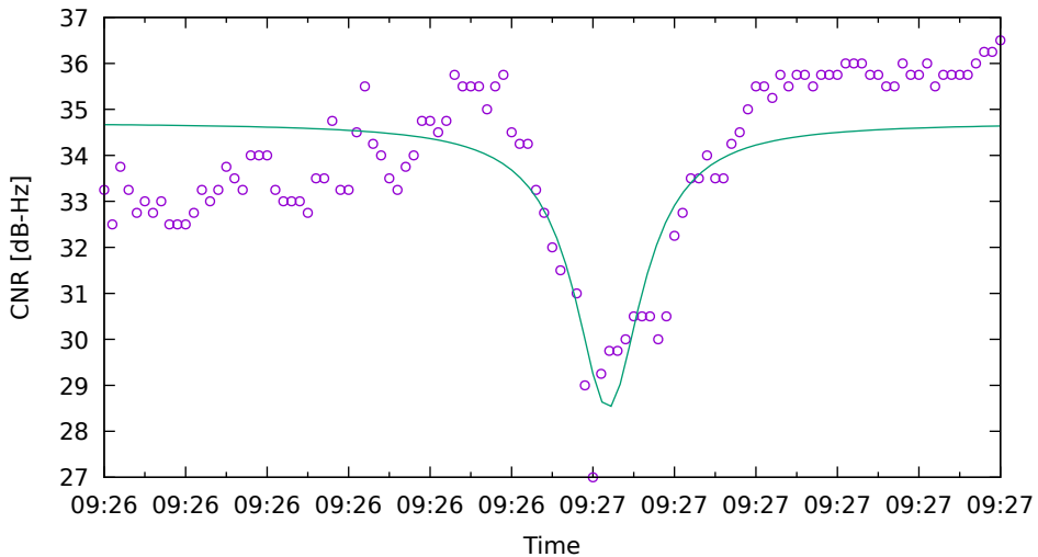
CNR fit for G08 on XiaomiMi8 - drive 6 (DOY262)
