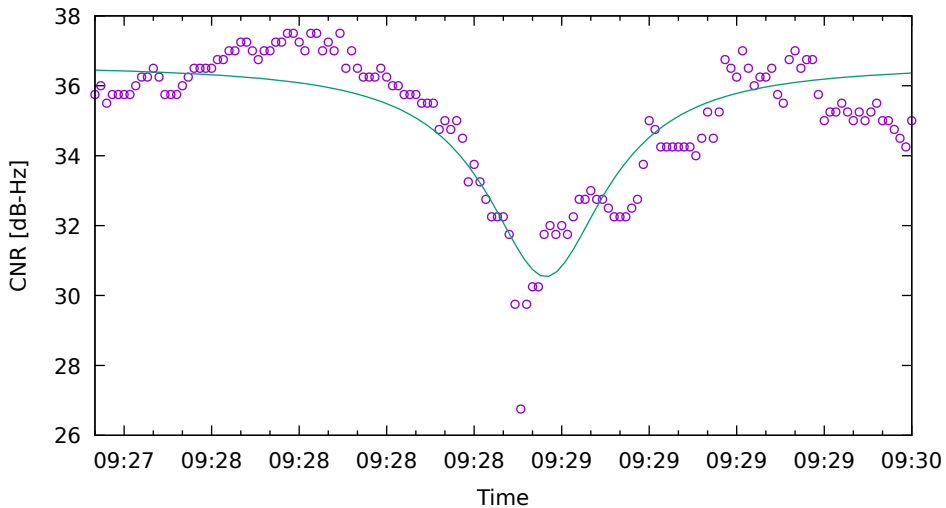
CNR fit for G08 on XiaomiMi8 - drive 7 (DOY262)
