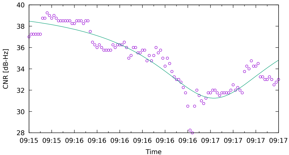
CNR fit for G17 on XiaomiMi8 - drive 1 (DOY262)
