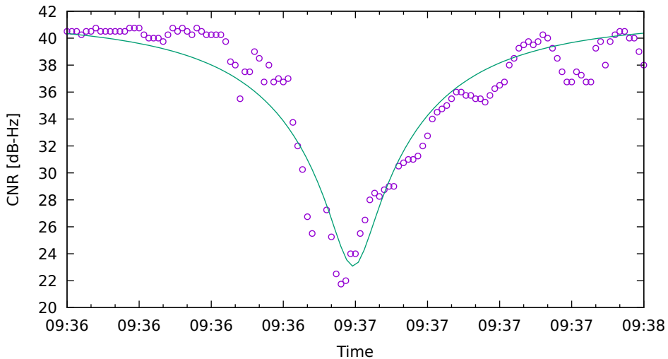
CNR fit for G17 on XiaomiMi8 - drive 11 (DOY262)
