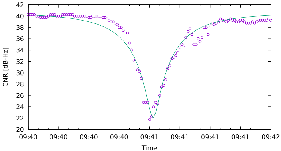
CNR fit for G17 on XiaomiMi8 - drive 13 (DOY262)
