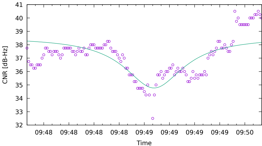
CNR fit for G17 on XiaomiMi8 - drive 17 (DOY262)
