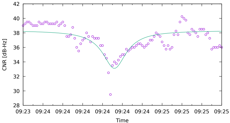
CNR fit for G17 on XiaomiMi8 - drive 5 (DOY262)
