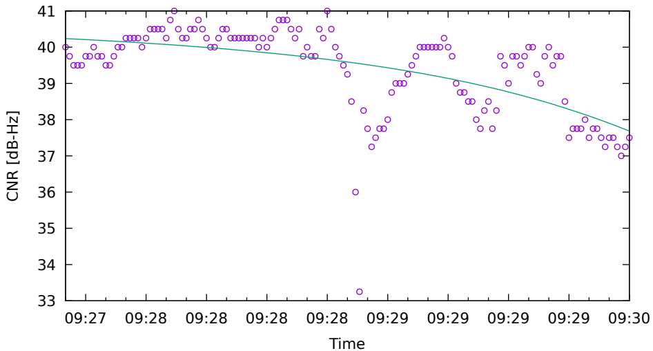
CNR fit for G17 on XiaomiMi8 - drive 7 (DOY262)
