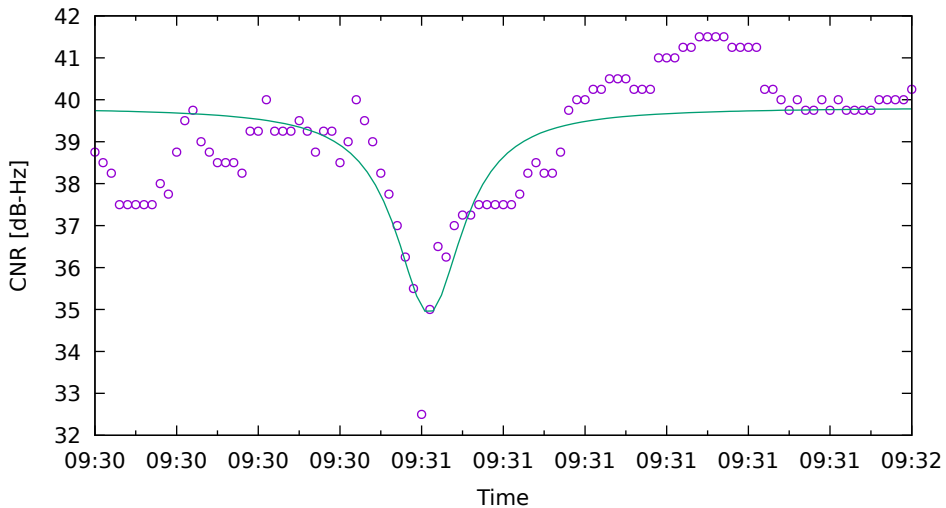
CNR fit for G17 on XiaomiMi8 - drive 8 (DOY262)
