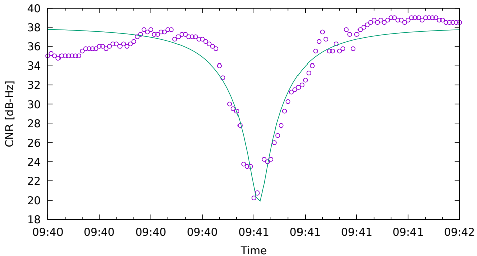
CNR fit for G19 on XiaomiMi8 - drive 13 (DOY262)
