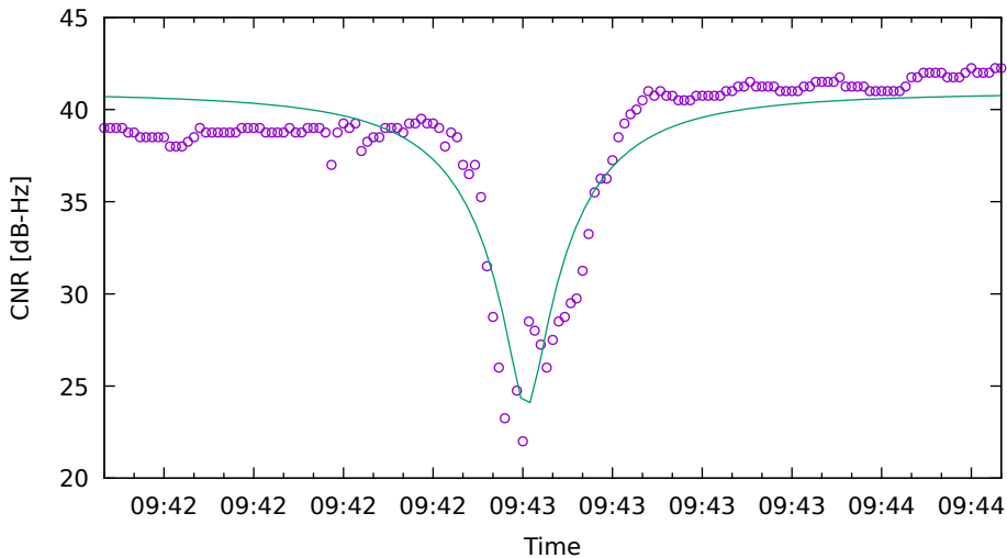
CNR fit for G19 on XiaomiMi8 - drive 14 (DOY262)
