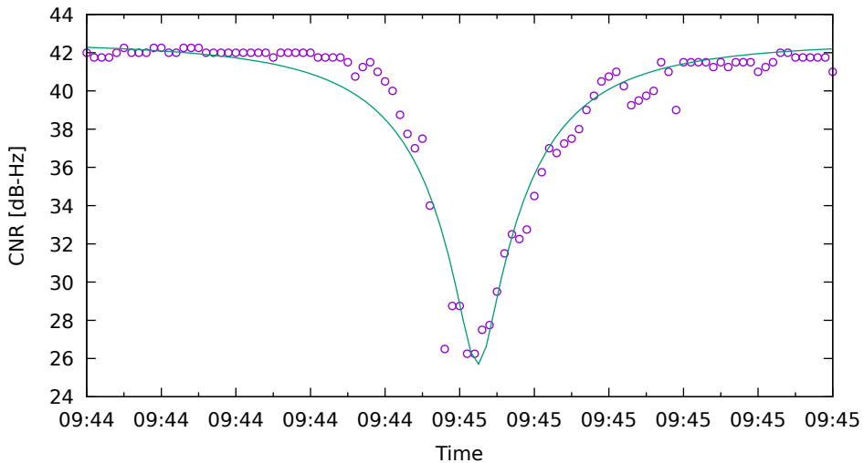
CNR fit for G19 on XiaomiMi8 - drive 15 (DOY262)
