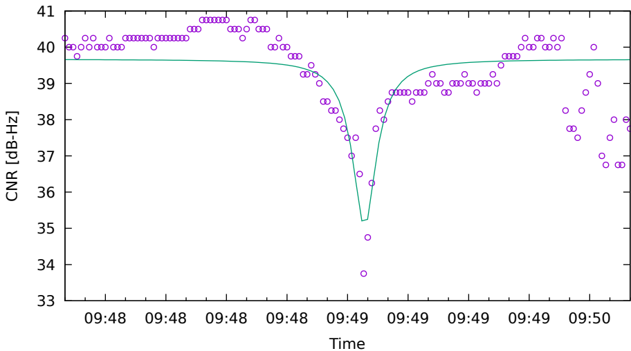
CNR fit for G19 on XiaomiMi8 - drive 17 (DOY262)
