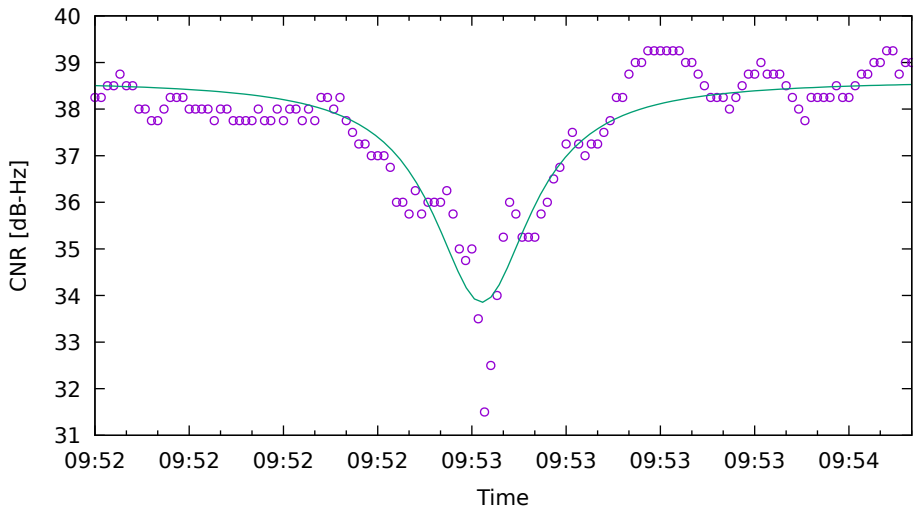
CNR fit for G19 on XiaomiMi8 - drive 19 (DOY262)
