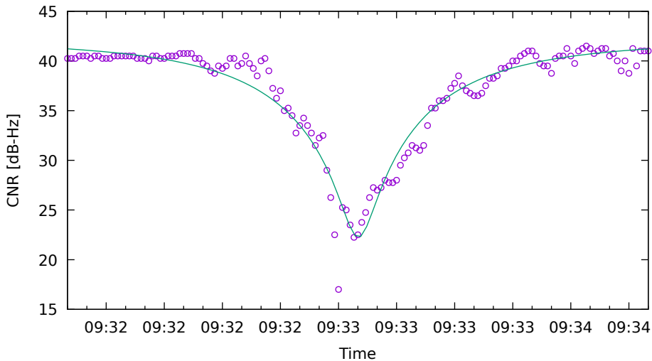
CNR fit for G19 on XiaomiMi8 - drive 9 (DOY262)
