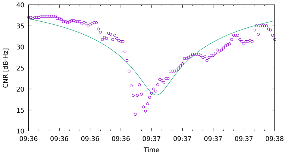
CNR fit for G21 on XiaomiMi8 - drive 11 (DOY262)
