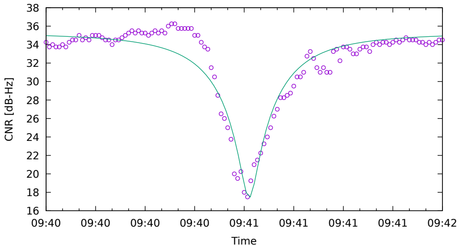
CNR fit for G21 on XiaomiMi8 - drive 13 (DOY262)
