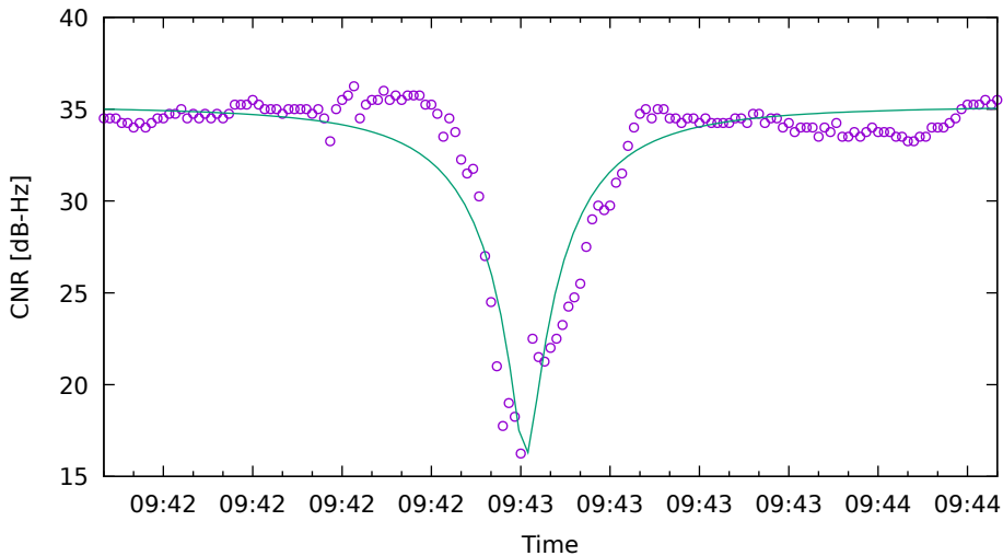
CNR fit for G21 on XiaomiMi8 - drive 14 (DOY262)
