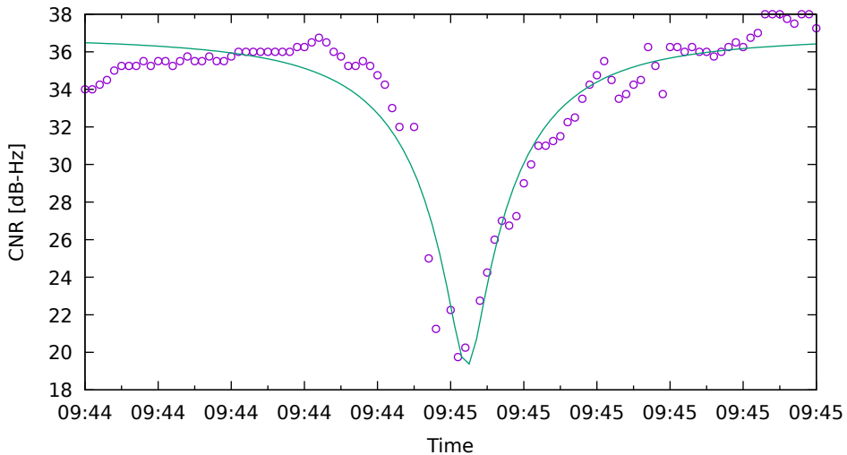
CNR fit for G21 on XiaomiMi8 - drive 15 (DOY262)
