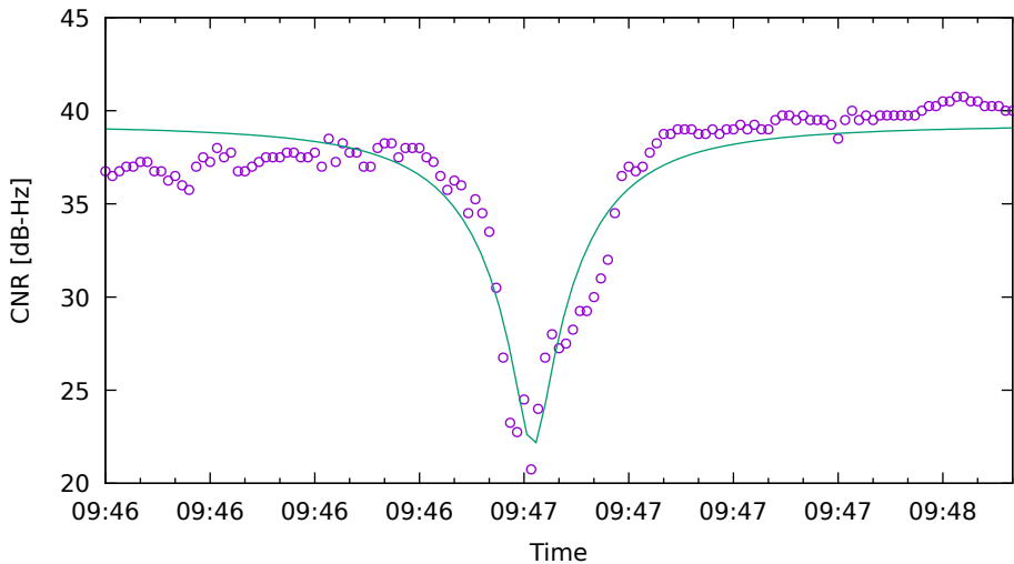
CNR fit for G21 on XiaomiMi8 - drive 16 (DOY262)
