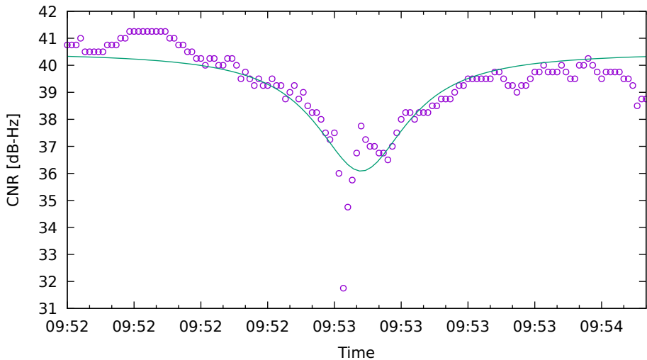
CNR fit for G21 on XiaomiMi8 - drive 19 (DOY262)
