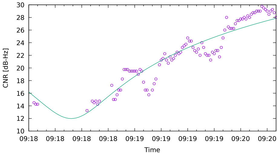
CNR fit for G21 on XiaomiMi8 - drive 2 (DOY262)
