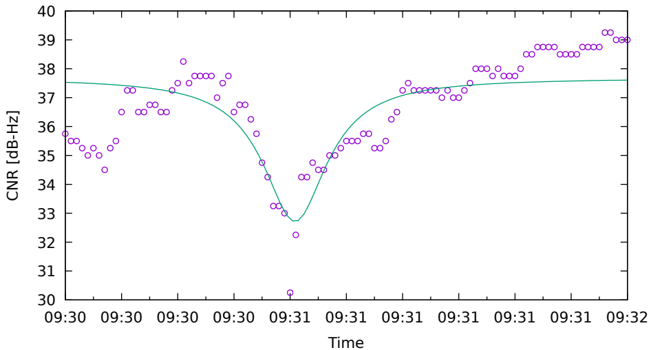
CNR fit for G21 on XiaomiMi8 - drive 8 (DOY262)
