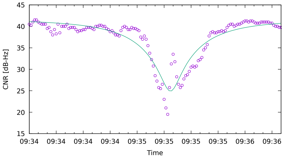
CNR fit for G22 on XiaomiMi8 - drive 10 (DOY262)
