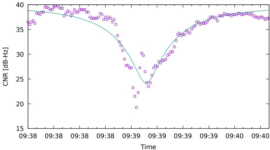
CNR fit for G22 on XiaomiMi8 - drive 12 (DOY262)
