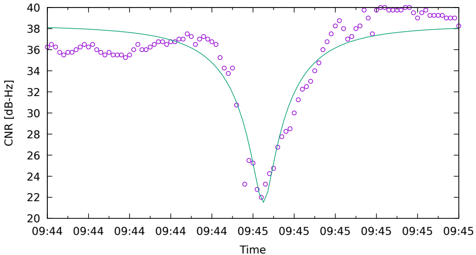
CNR fit for G22 on XiaomiMi8 - drive 15 (DOY262)
