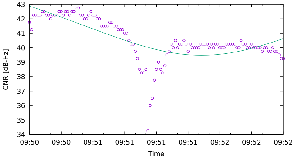
CNR fit for G22 on XiaomiMi8 - drive 18 (DOY262)
