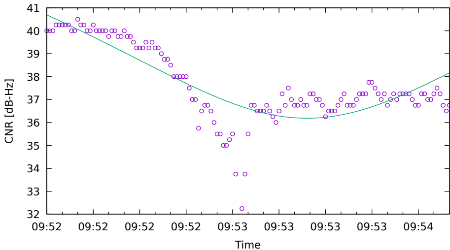
CNR fit for G22 on XiaomiMi8 - drive 19 (DOY262)
