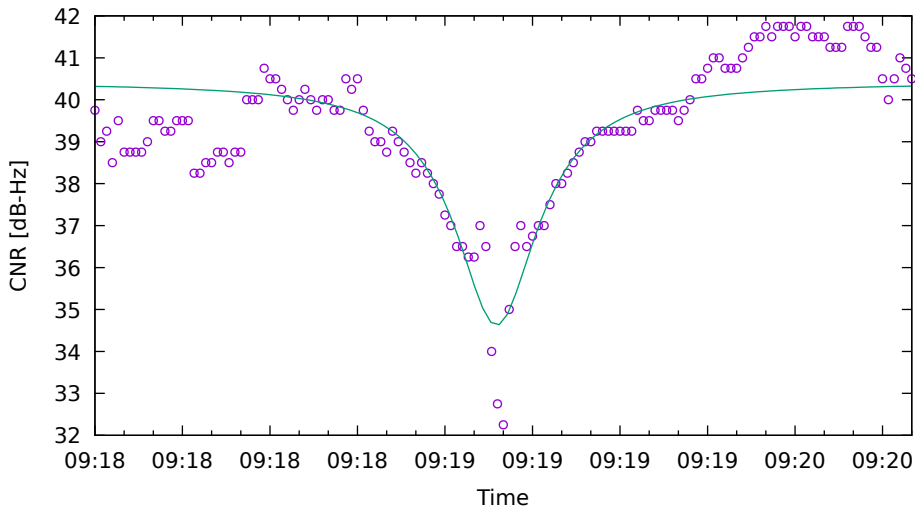
CNR fit for G22 on XiaomiMi8 - drive 2 (DOY262)
