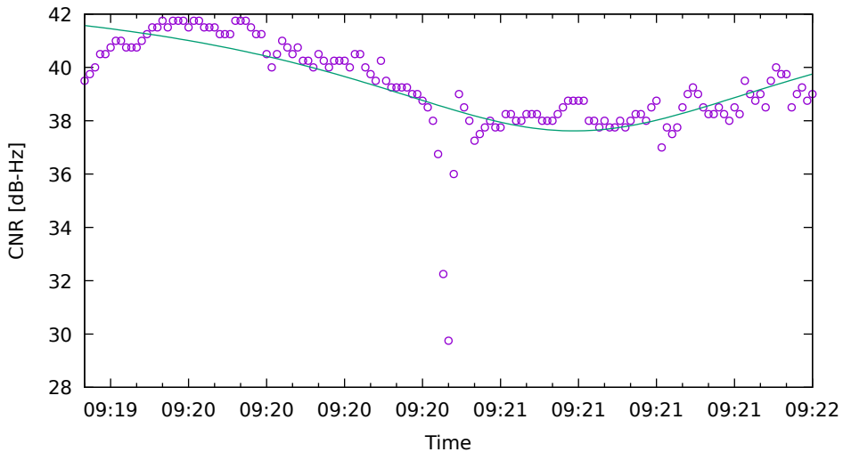
CNR fit for G22 on XiaomiMi8 - drive 3 (DOY262)
