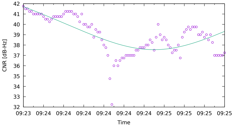
CNR fit for G22 on XiaomiMi8 - drive 5 (DOY262)
