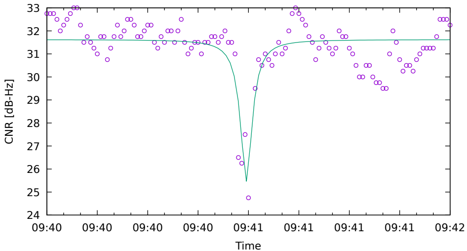
CNR fit for R07 on XiaomiMi8 - drive 13 (DOY262)
