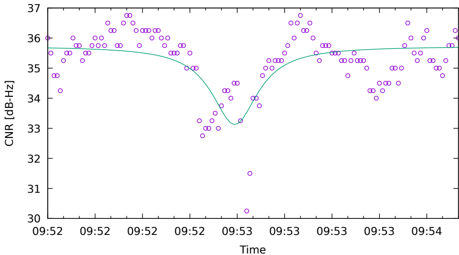
CNR fit for R07 on XiaomiMi8 - drive 19 (DOY262)
