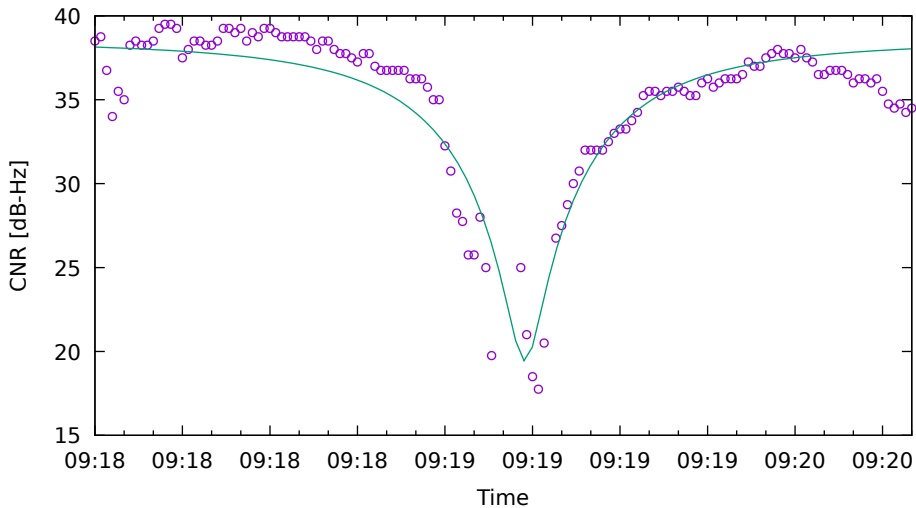
CNR fit for R07 on XiaomiMi8 - drive 2 (DOY262)
