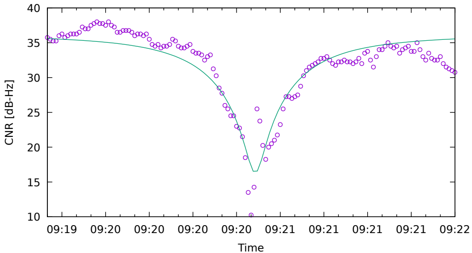
CNR fit for R07 on XiaomiMi8 - drive 3 (DOY262)
