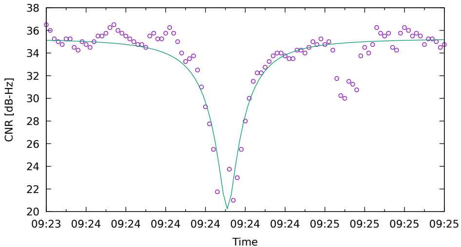
CNR fit for R07 on XiaomiMi8 - drive 5 (DOY262)
