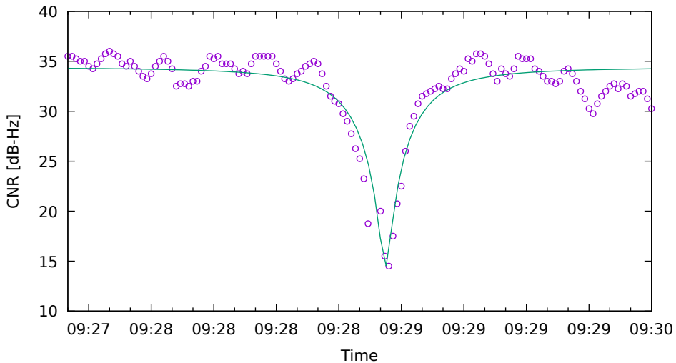
CNR fit for R07 on XiaomiMi8 - drive 7 (DOY262)
