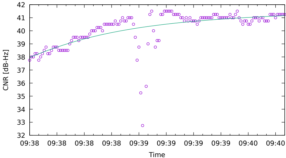
CNR fit for R24 on XiaomiMi8 - drive 12 (DOY262)
