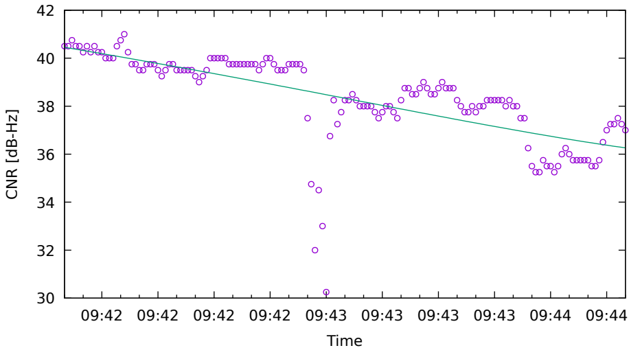
CNR fit for R24 on XiaomiMi8 - drive 14 (DOY262)
