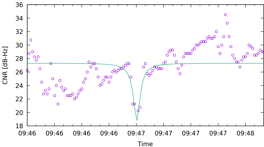
CNR fit for R24 on XiaomiMi8 - drive 16 (DOY262)
