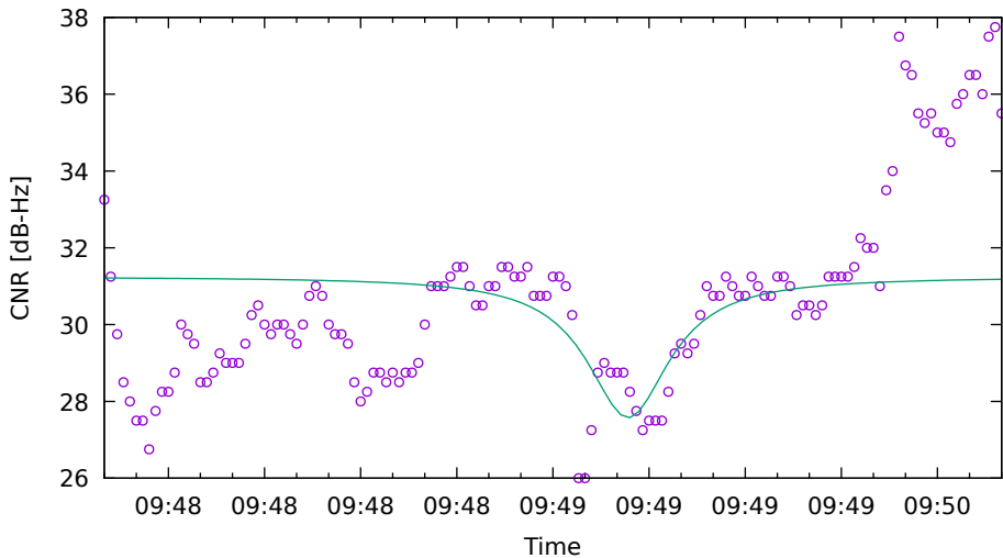
CNR fit for R24 on XiaomiMi8 - drive 17 (DOY262)
