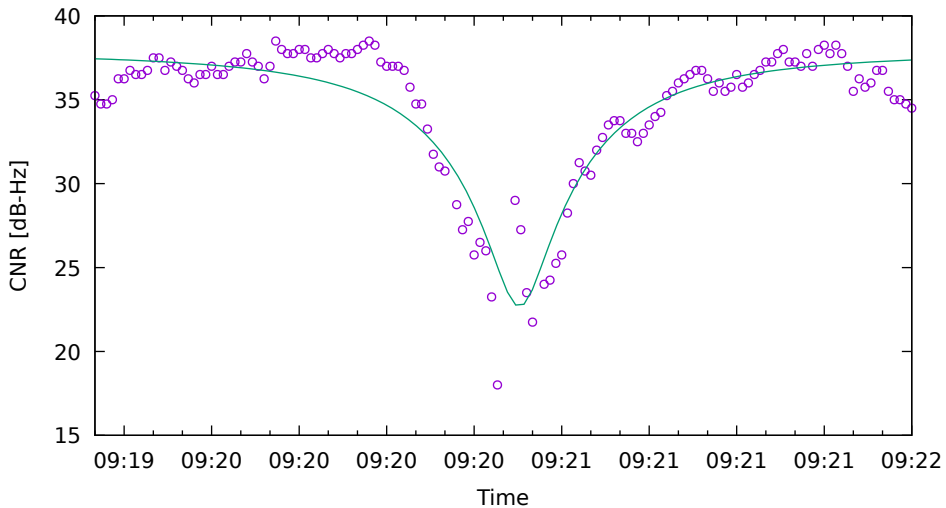
CNR fit for R24 on XiaomiMi8 - drive 3 (DOY262)
