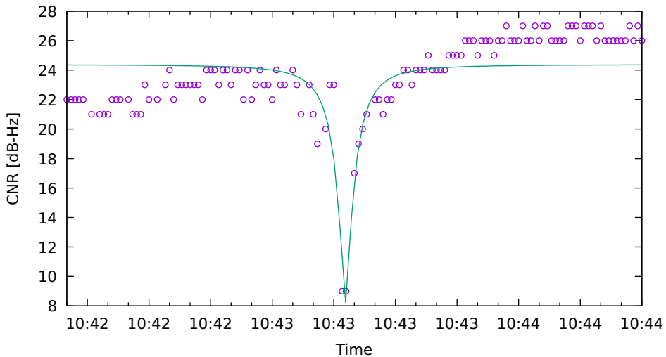
CNR fit for C06 on HuaweiP40 - drive 1 (DOY262)
