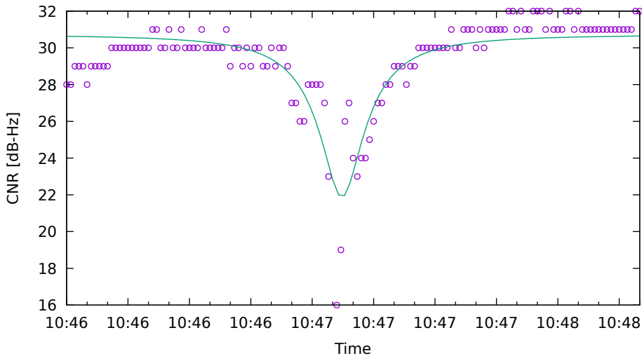
CNR fit for C06 on HuaweiP40 - drive 3 (DOY262)
