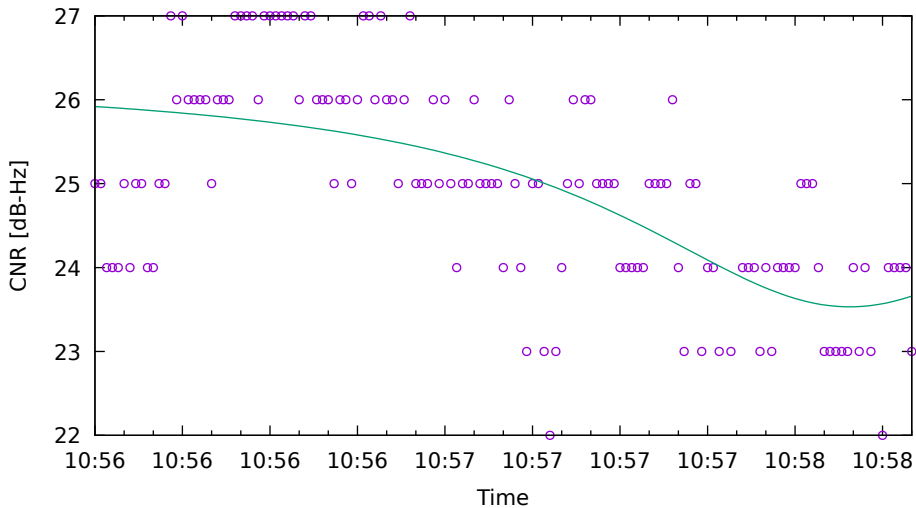
CNR fit for C09 on HuaweiP40 - drive 8 (DOY262)
