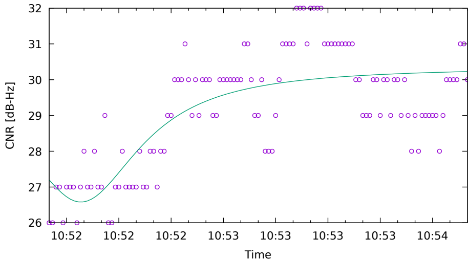
CNR fit for C14 on HuaweiP40 - drive 6 (DOY262)
