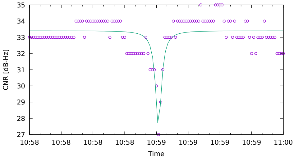
CNR fit for C14 on HuaweiP40 - drive 9 (DOY262)
